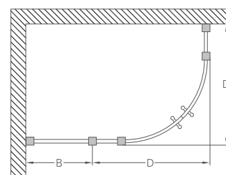
Right Handed
