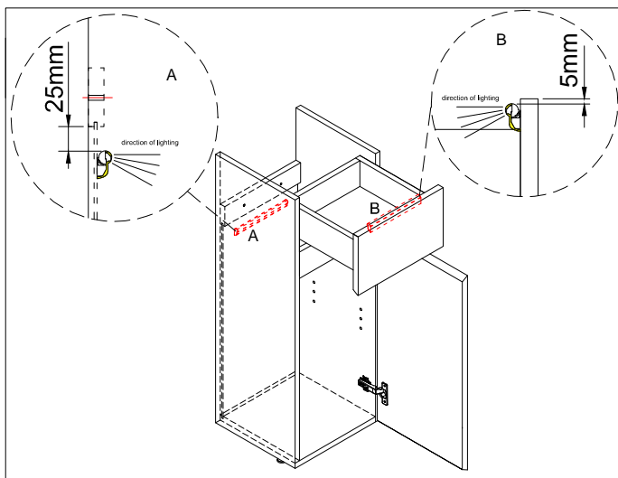
1: The above diagram shows the recommended installation position for drawer units and cabinets.
