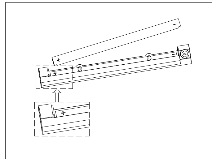
6: Click the battery holder onto the LED light body. Ensure the +/- signs are consistent with the light body.
