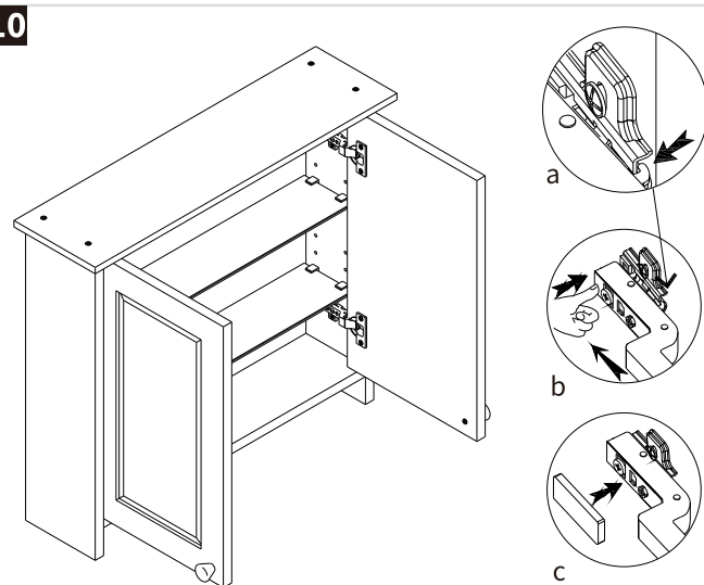
Mounting cabinet door
