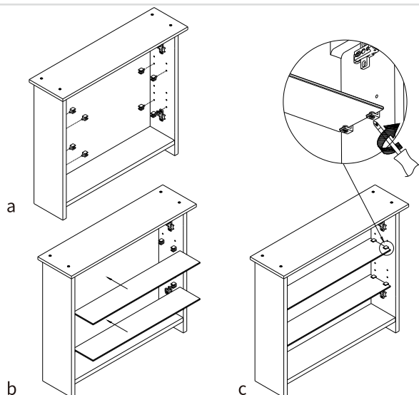
Install glass shelves
