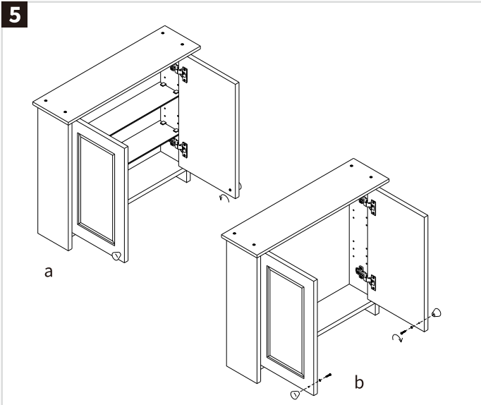
Install the handle facing outward
