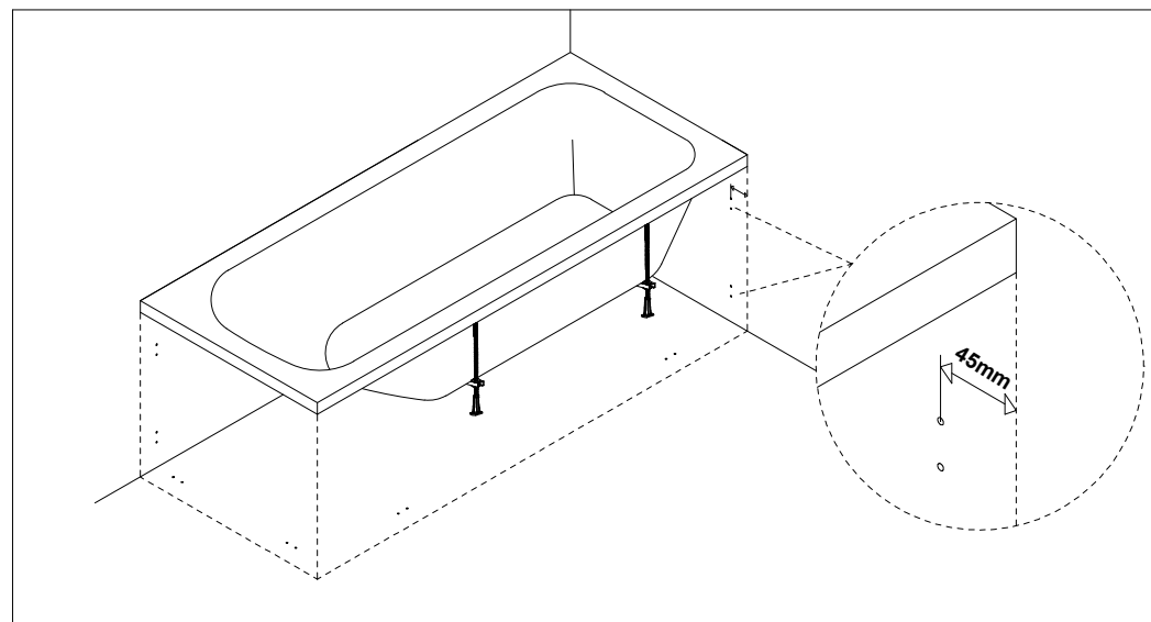
14: Mark the hole positions on the wall and floor, then drill the holes to fix the L brackets.
