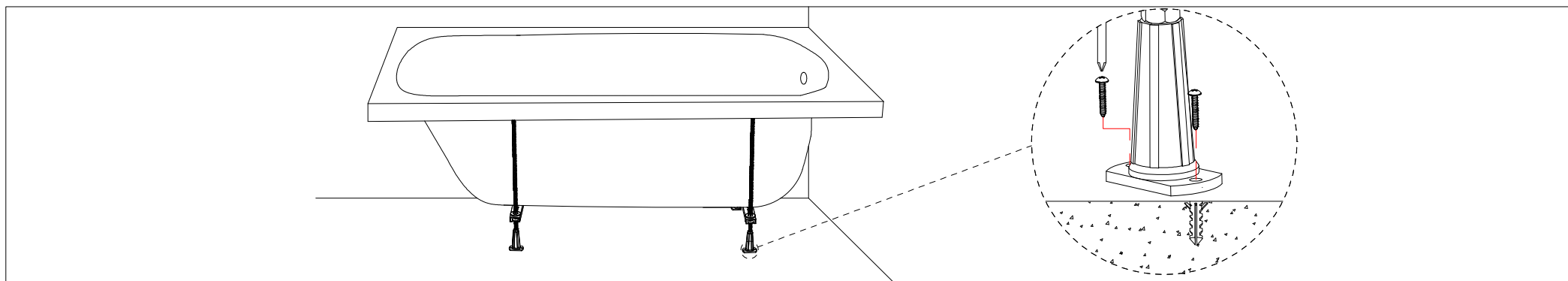
12: It is essential that once the bath is in its final position the bath legs be firmly fixed to and secured to the floor using fixings appropriate for the type of floor surface (such fixing not included)
